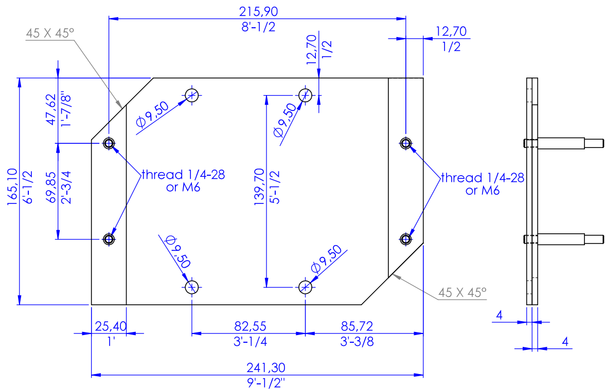
Mounting plate for TUAAM in rear mount with panel generator n°9 MK3 FV 546131
