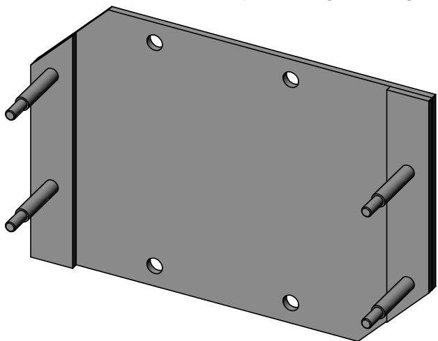
Mounting plate for TUAAM in rear mount with panel generator n°9 MK3 FV 546131
