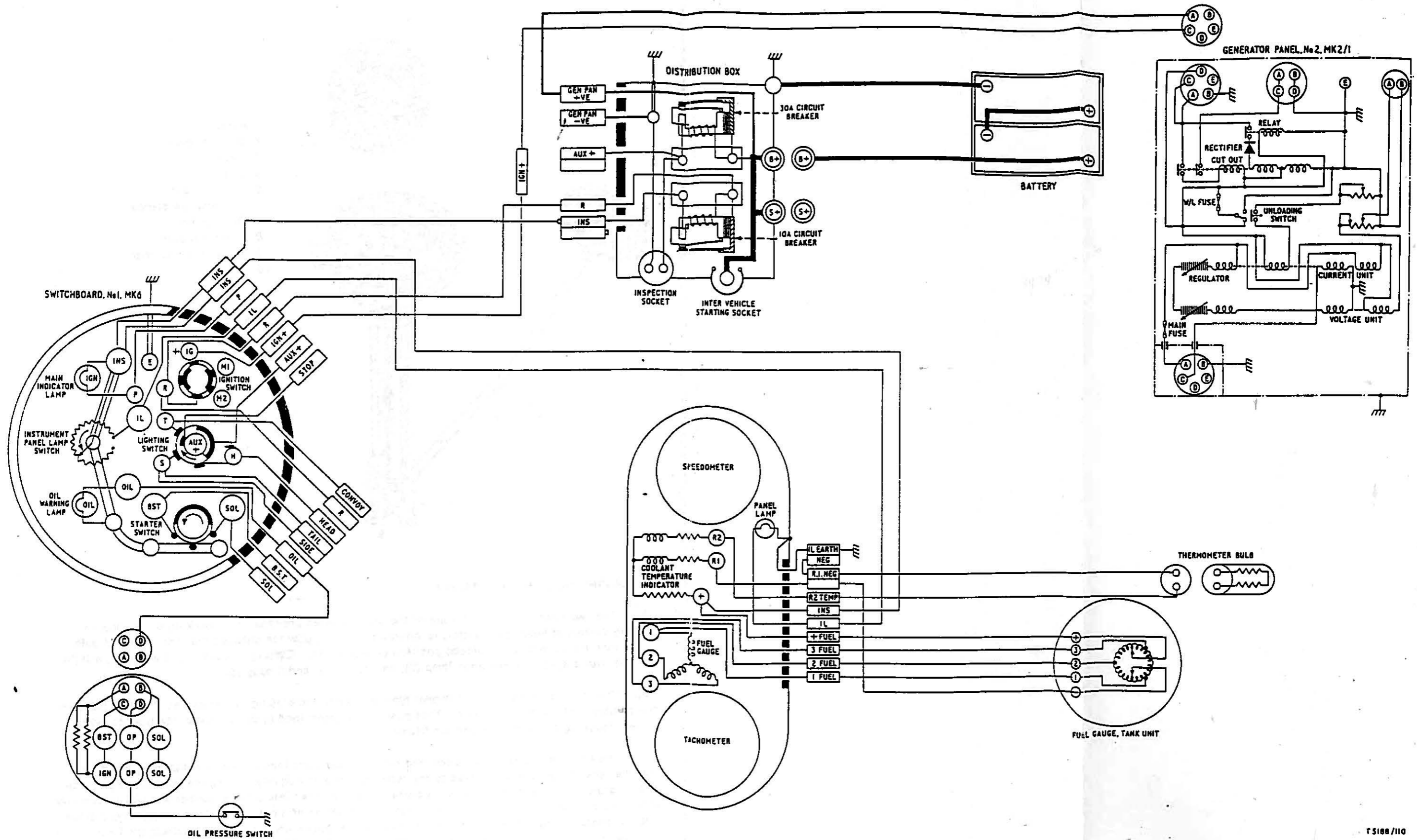
Fig 25 Instruments wiring diagram (red)
