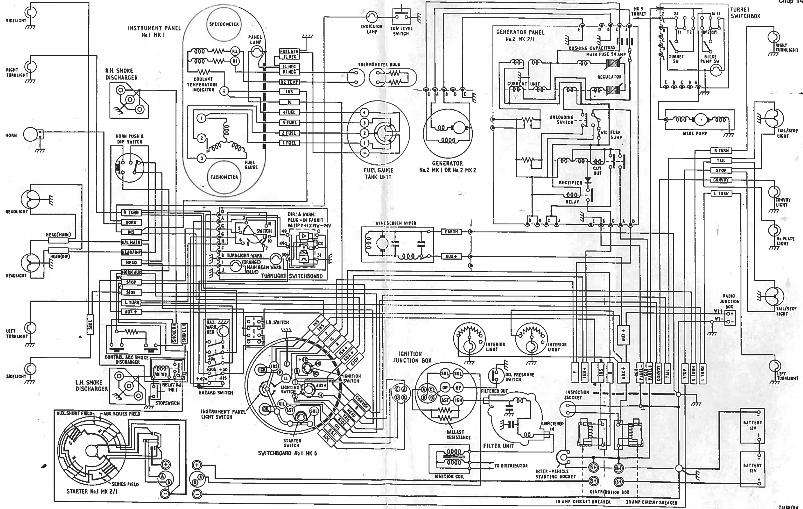
Fig 1 Vehicle wiring diagram
